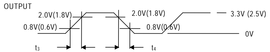
All Outputs Rise/Fall Time
