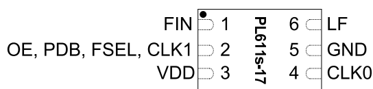
DFN-6L (2.0 x 1.3 x 0.6mm)
