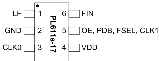
SOT23-6L (3.0 x 3.0 x 1.35mm)
