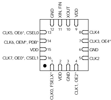
QFN Package
